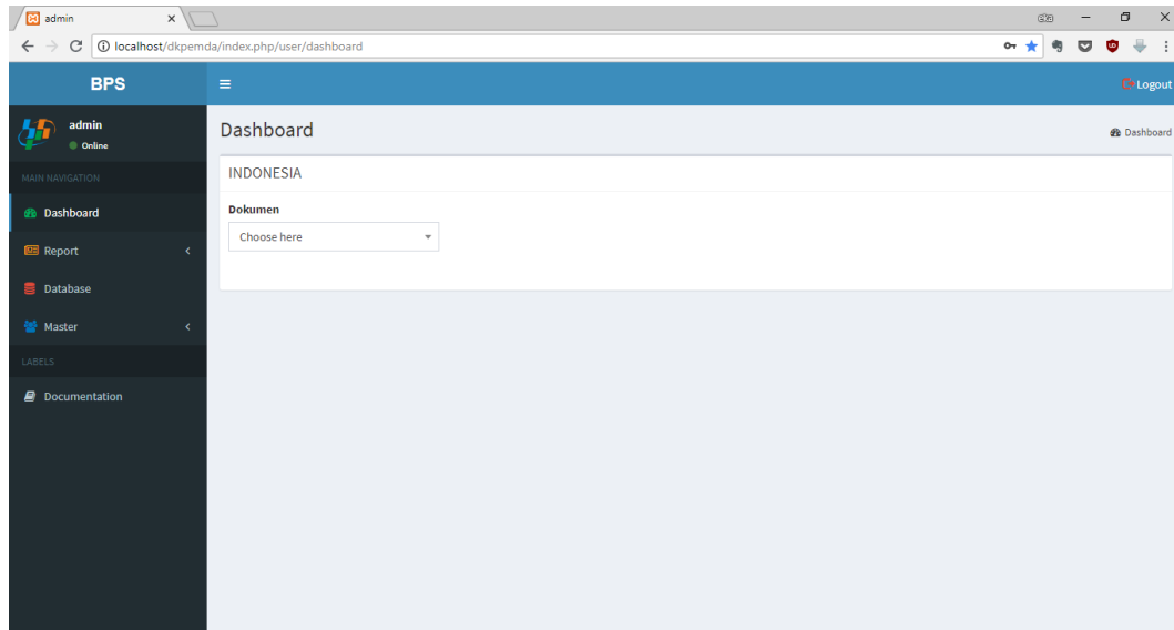
Gambar 19. Halaman admin
